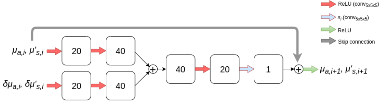
Figure 1: Diagram of one CNN denoted as G_{\theta_i} , representing one iteration of the deep Gauss-Newton. The red arrows denote a convolutional layer with 5 \times 5 kernel for a 2D image (or 5 \times 5 \times 5 kernel for a 3D image), bias and followed by a ReLU. The resulting channels in each layer are indicated in the squares. The blue arrow denotes a convolutional layer followed by a scalar multiplication. The residual update (by the skip connection) is then projected to the positive numbers by the last ReLU (shown as green arrow).
