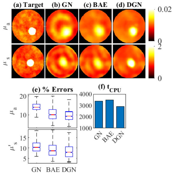
Figure 8: Reconstructions of mix targets in the presence of modelling errors. (a) Target absorption \mu_a and scattering \mu_s , (b) estimates using GN, (c) BAE, and (d) DGN. Artefacts due to modelling errors are seen in the GN estimates. These are compensated in the BAE and DGN estimates. Statistics of the estimation errors for 1000 evaluation cases are shown in (e), and the evaluation times in (f).
